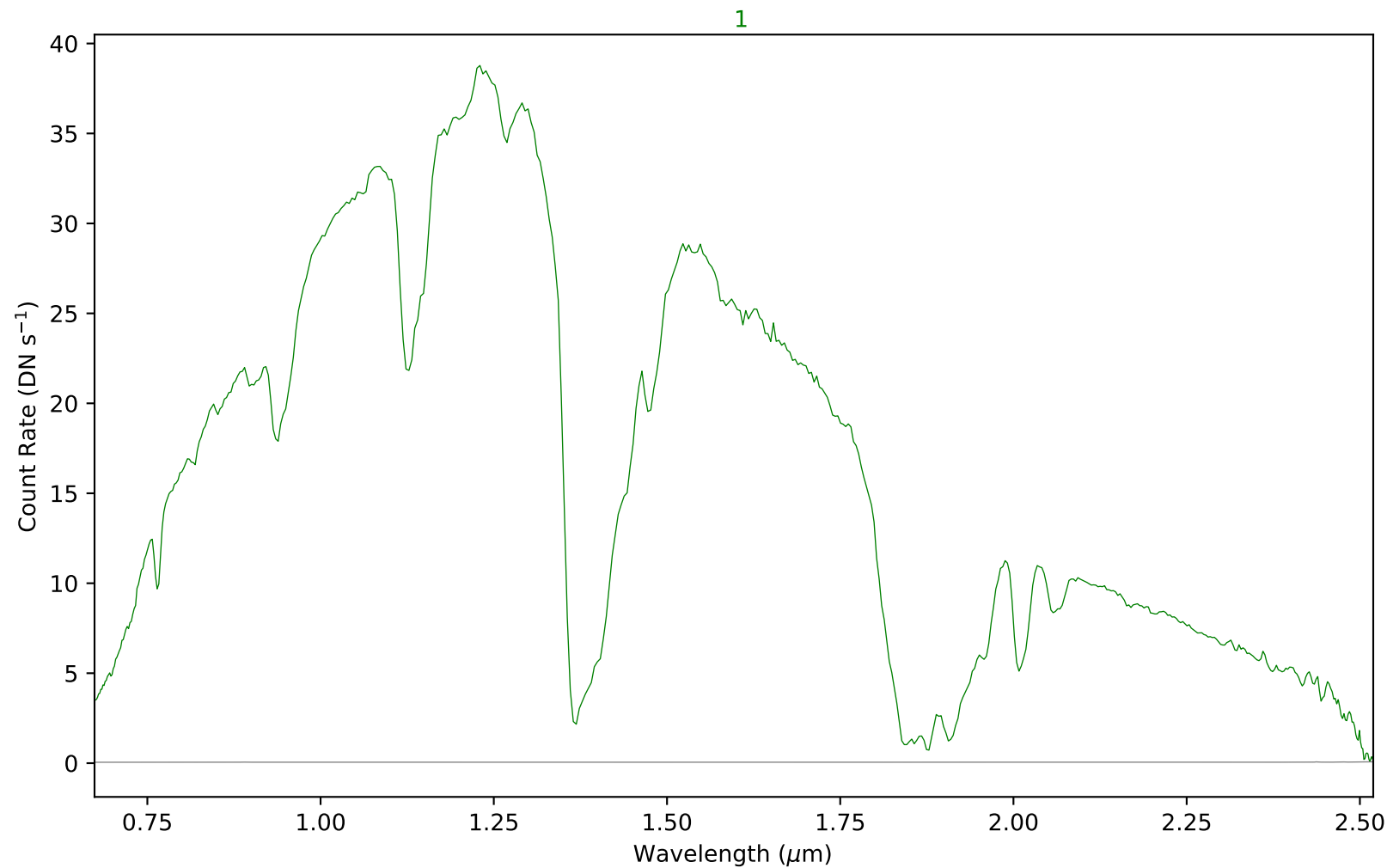
combspec232-243.fits - Aperture 1
