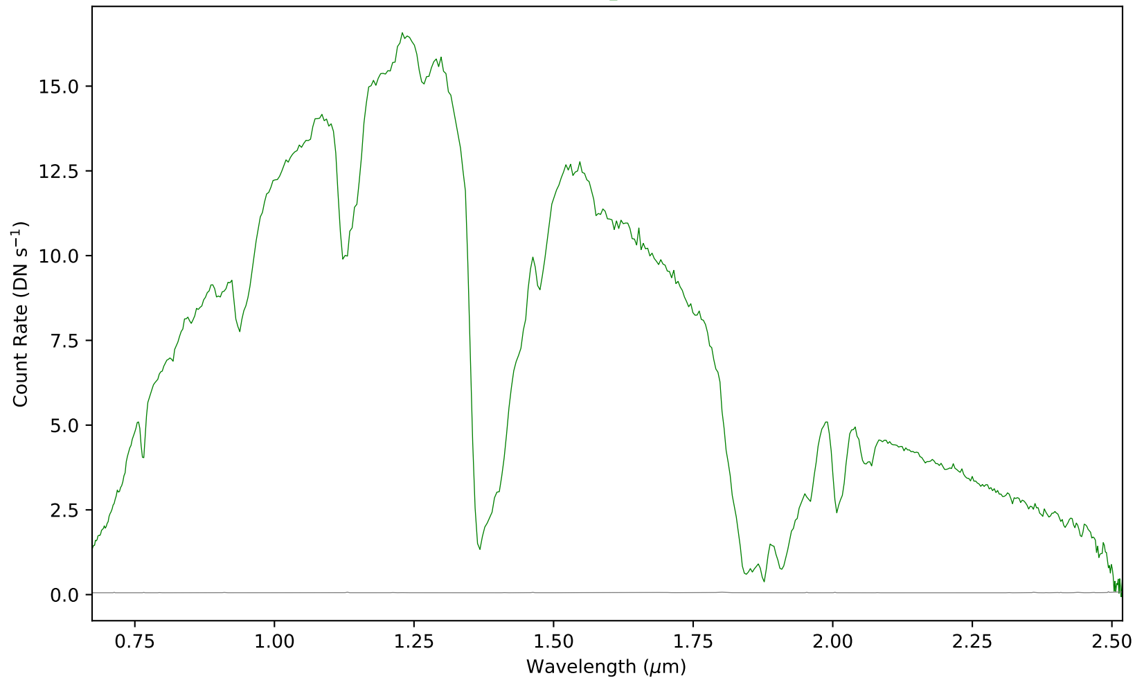
combspec268-279.fits - Aperture 1
