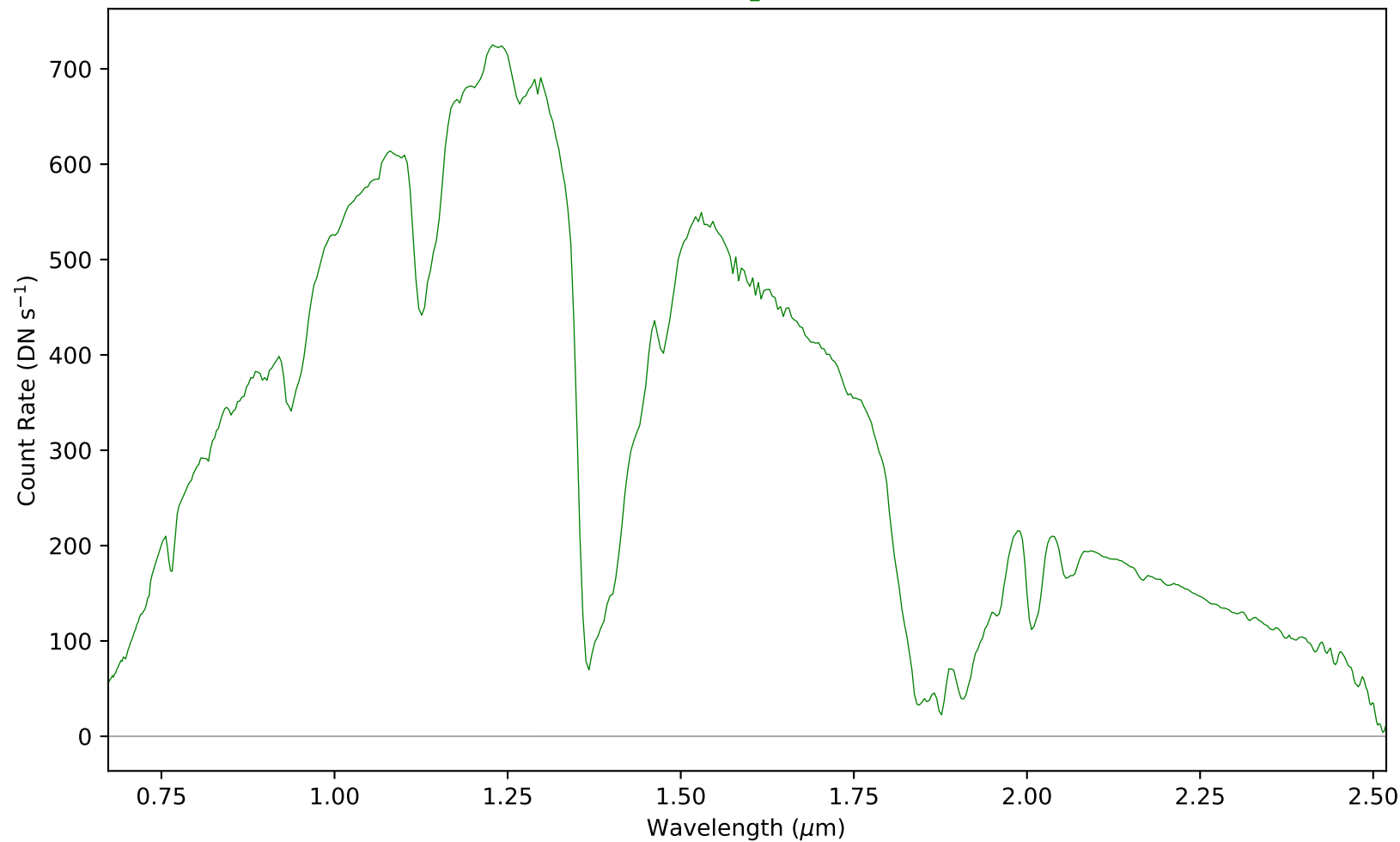
combspec288-397.fits - Aperture 1
