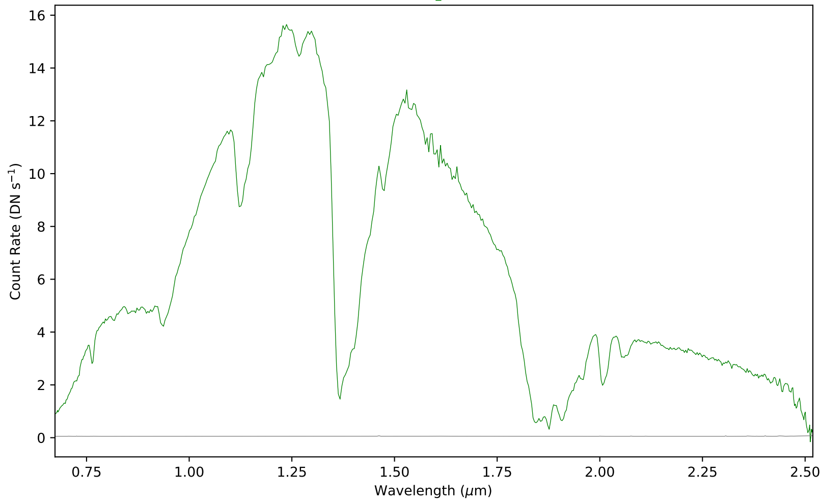
combspec312-323.fits - Aperture 1
