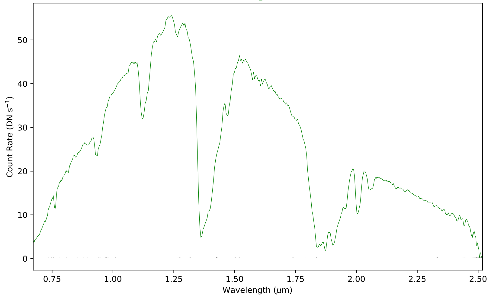
combspec380-385.fits - Aperture 1
