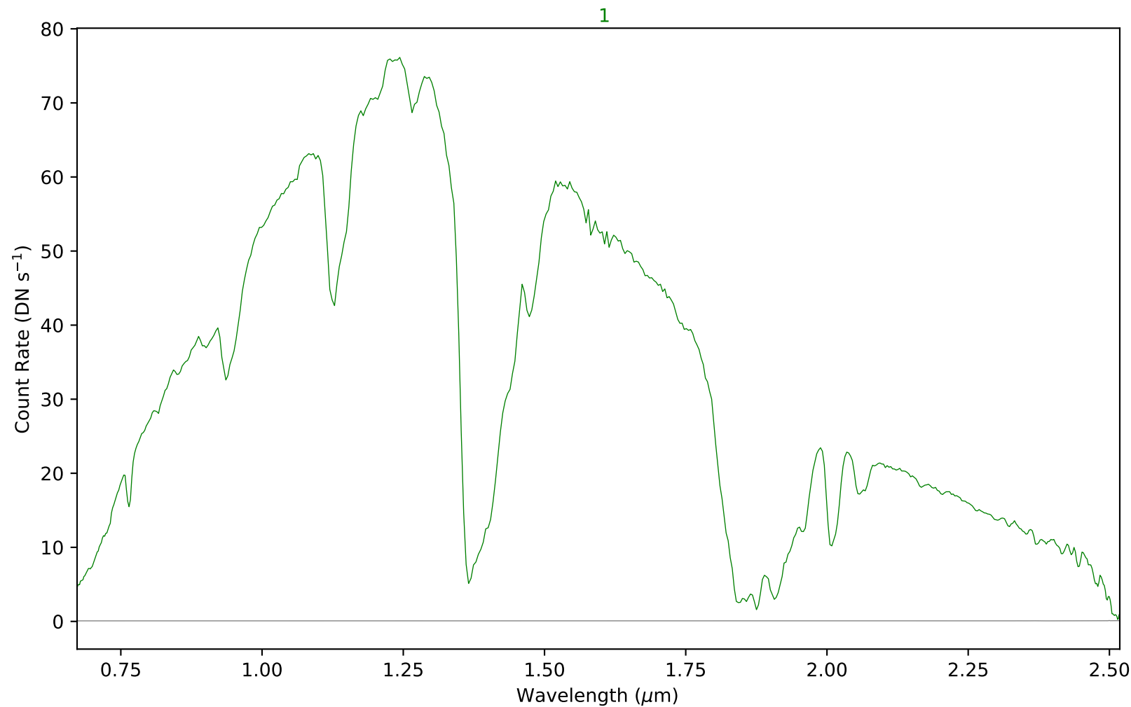
combspec398-407.fits - Aperture 1
