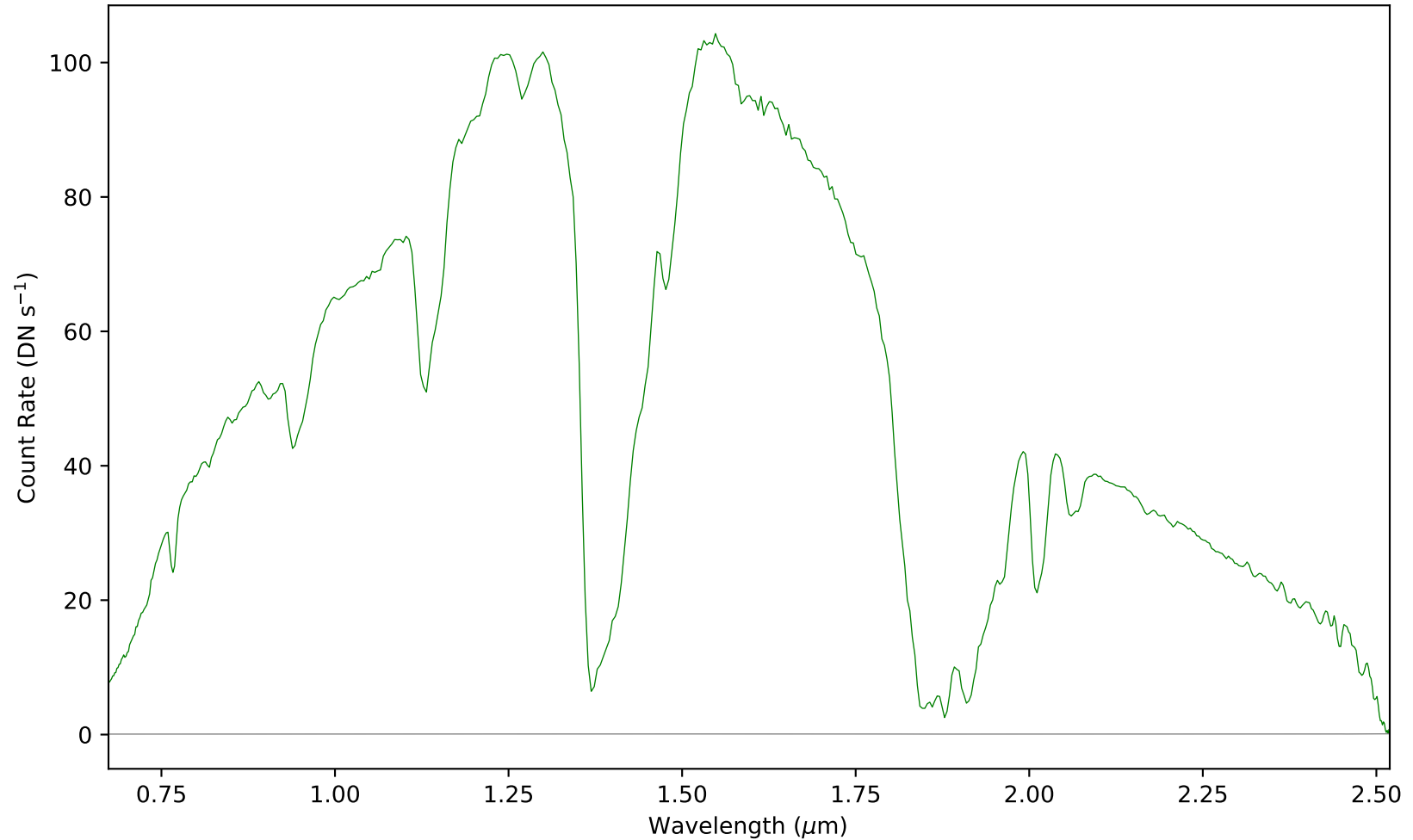
combspec40-51.fits - Aperture 1
