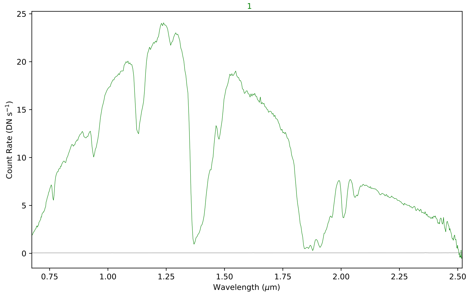
combspec82-95.fits - Aperture 1
