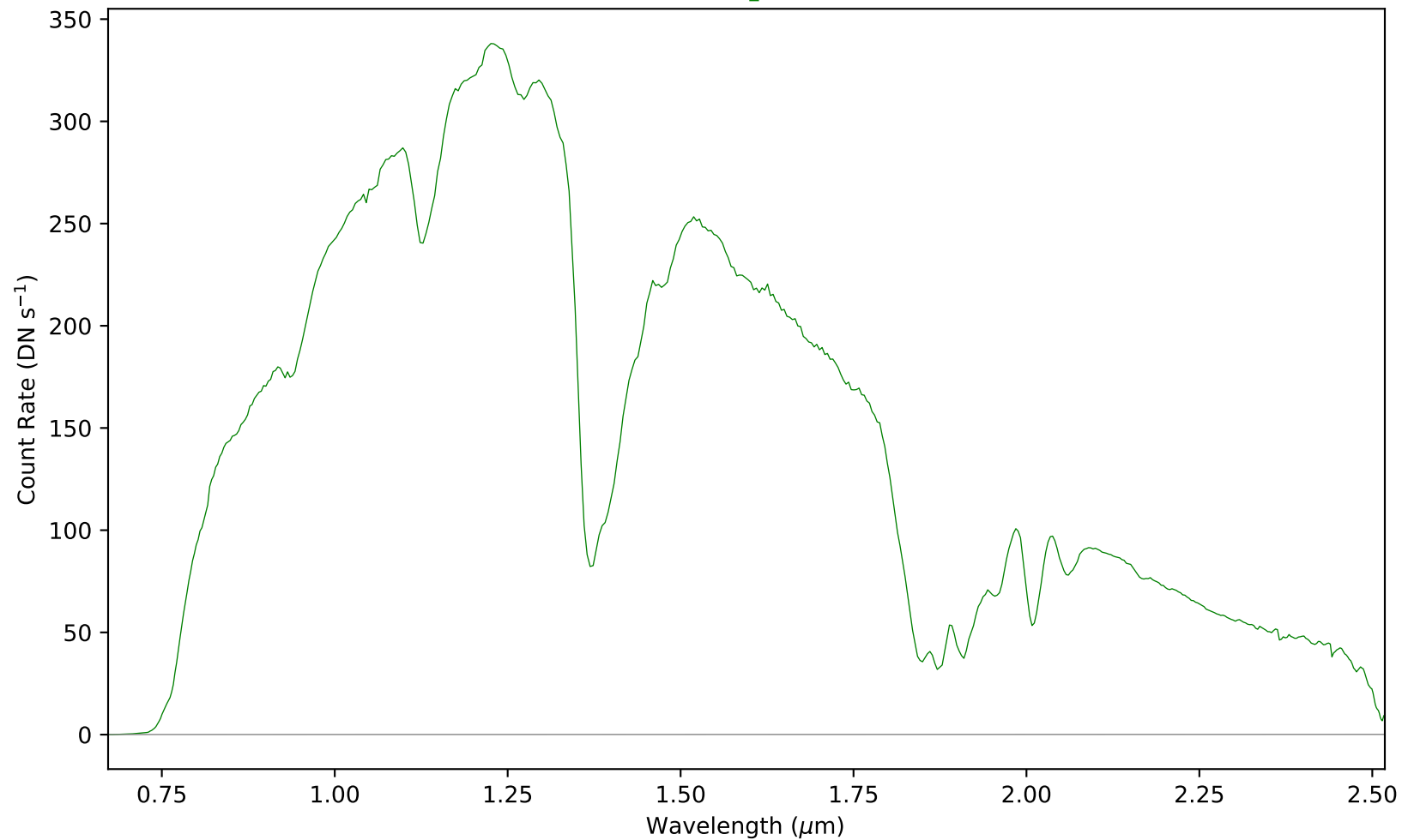
combspec1001-1010.fits - Aperture 1
