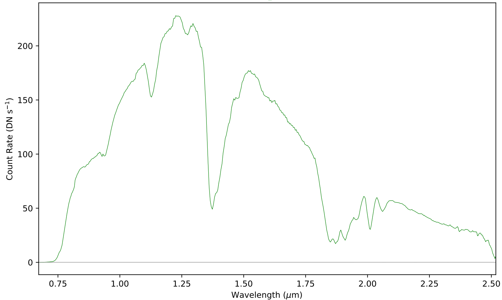
combspec1011-1024.fits - Aperture 1
