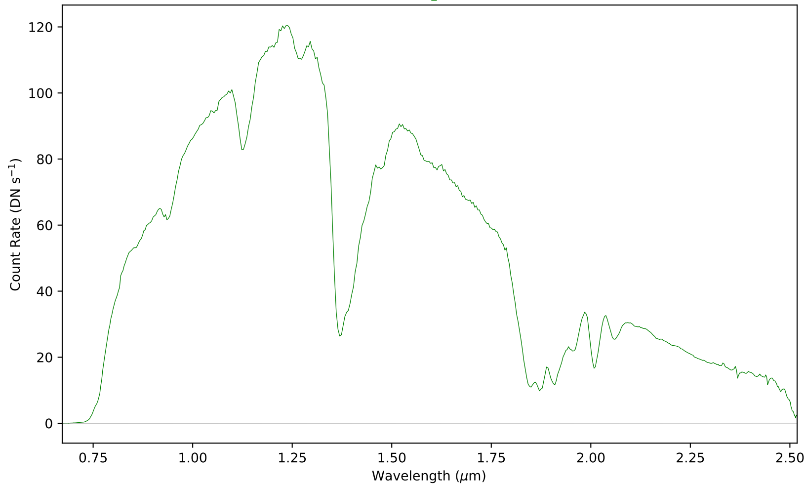
combspec1031-1044.fits - Aperture 1
