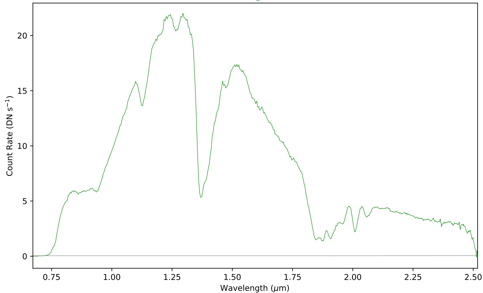
combspec1045-1058.fits - Aperture 1
