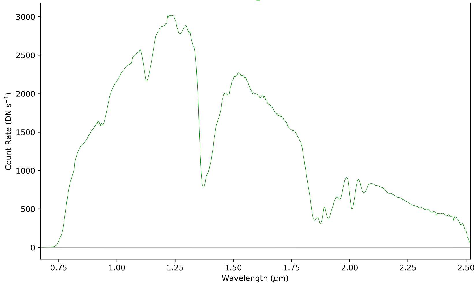
combspec1059-1068.fits - Aperture 1
