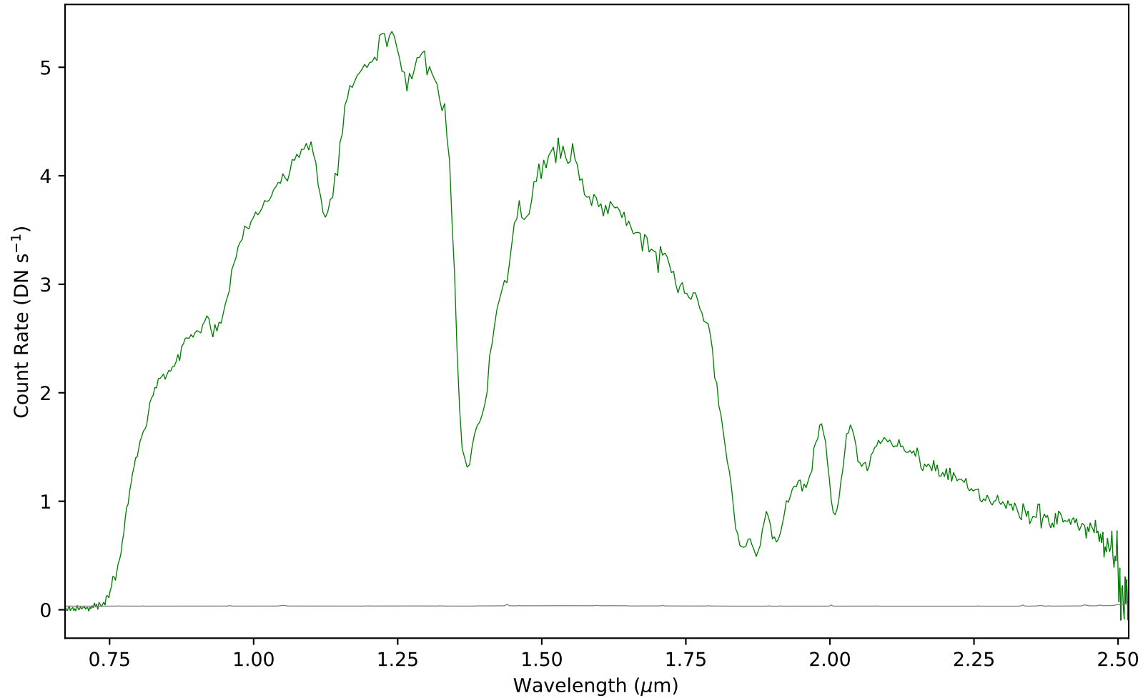
combspec1069-1084.fits - Aperture 1
