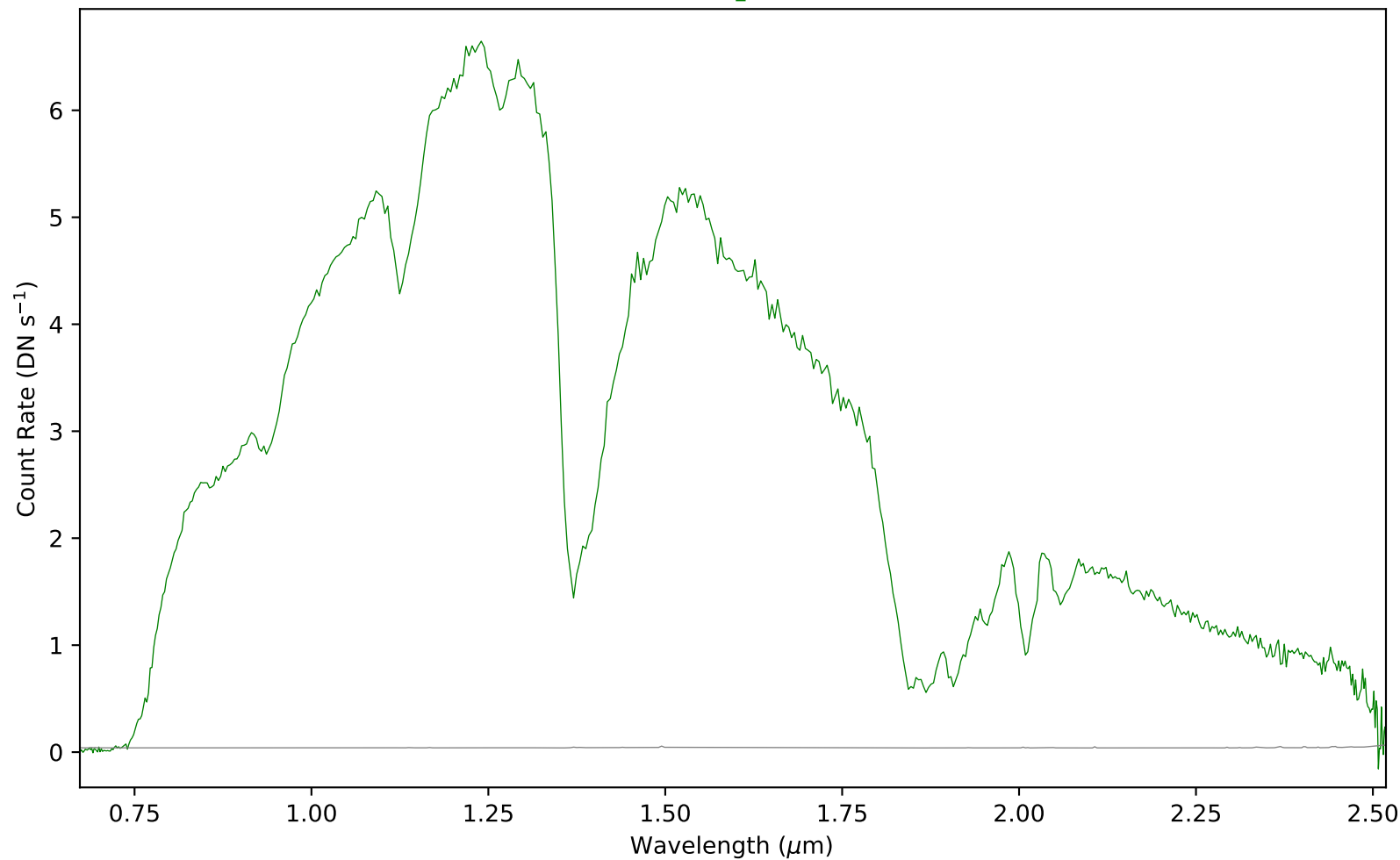
combspec1091-1104.fits - Aperture 1
