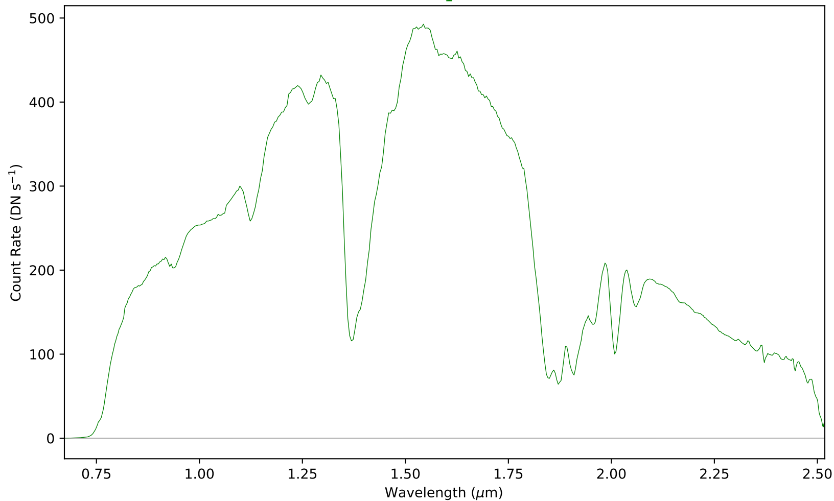
combspec1119-1132.fits - Aperture 1
