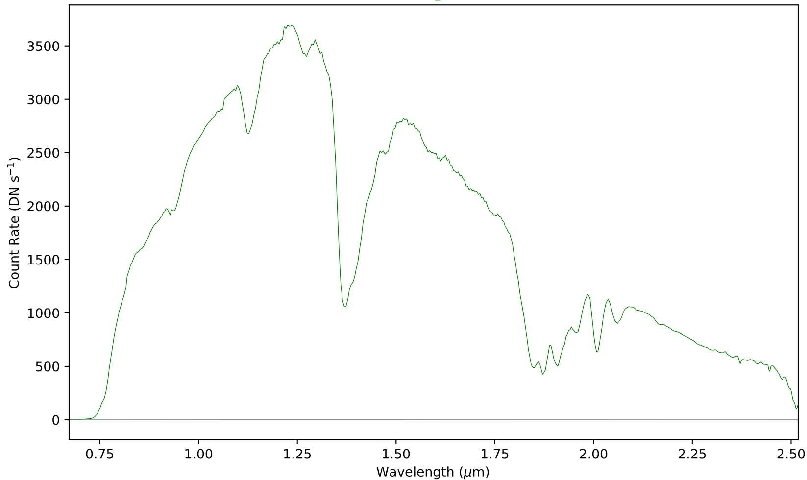
combspec1133-1142.fits - Aperture 1
