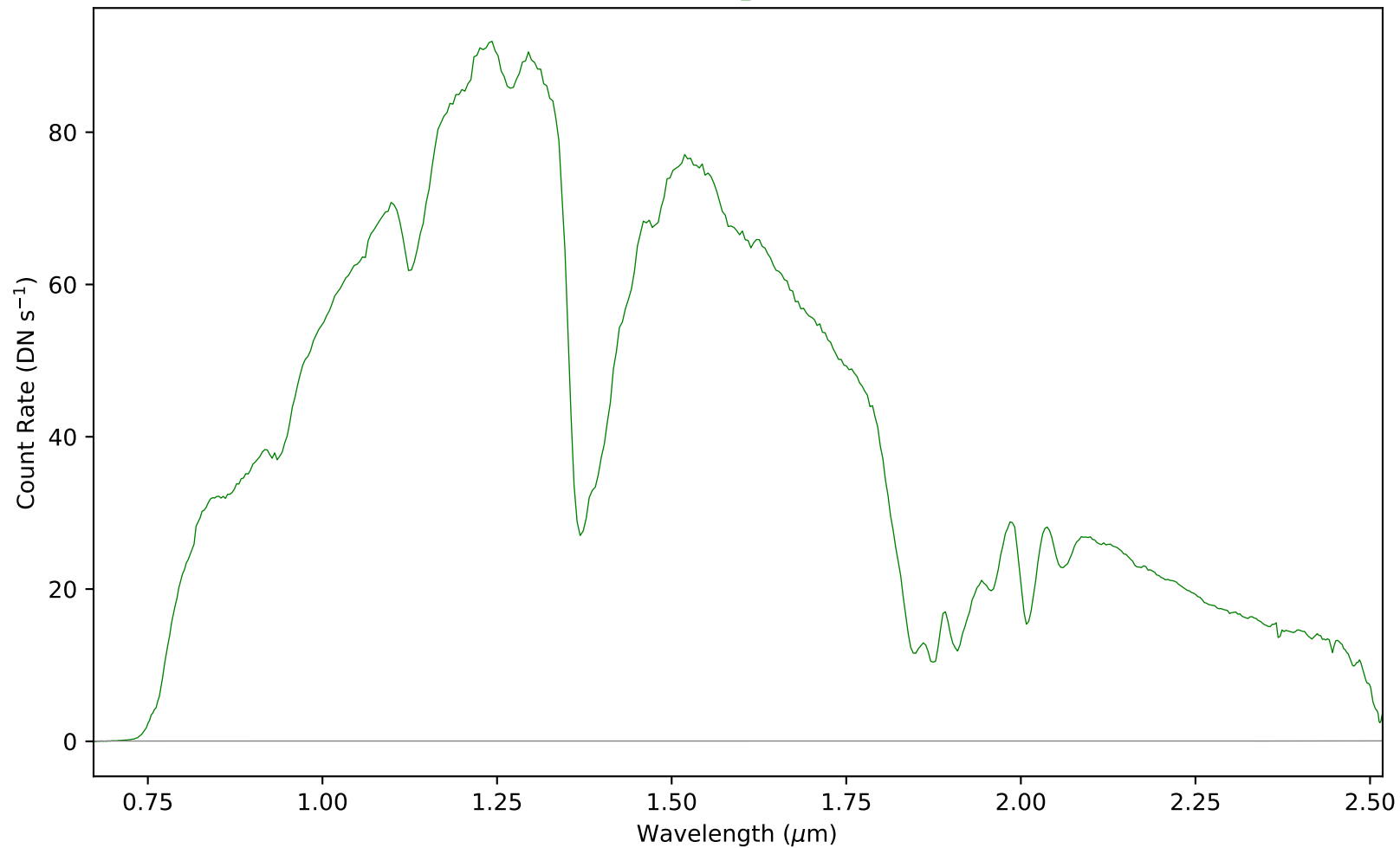
combspec1149-1162.fits - Aperture 1
