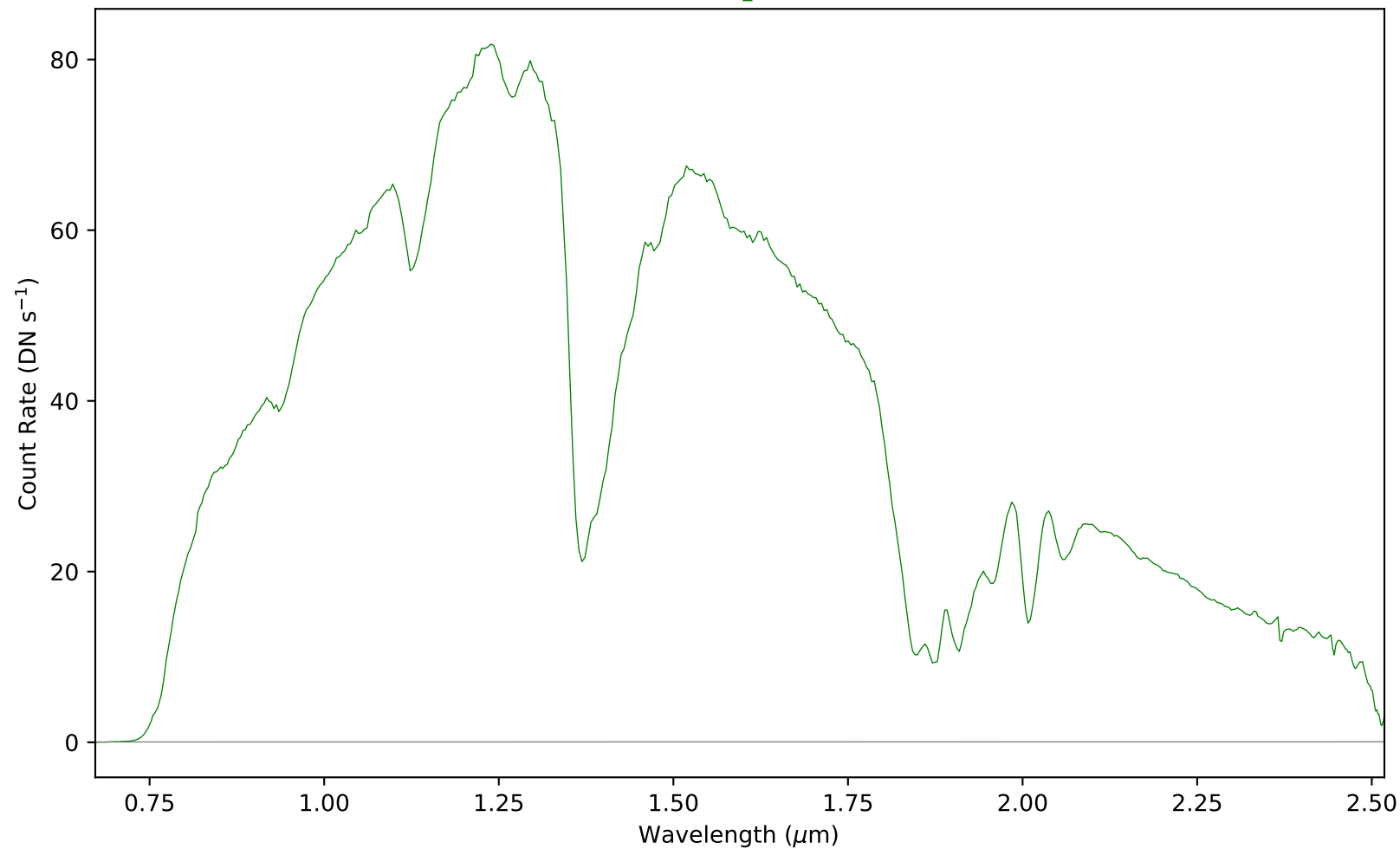
combspec1163-1176.fits - Aperture 1
