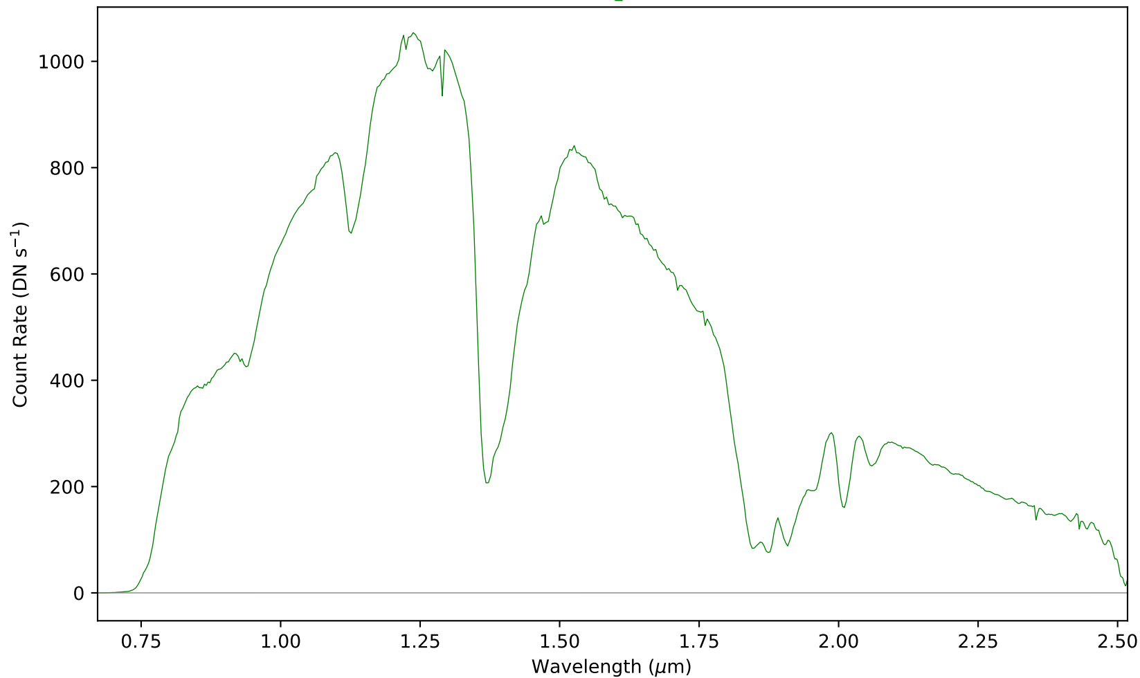
combspec2017-2030.fits - Aperture 1
