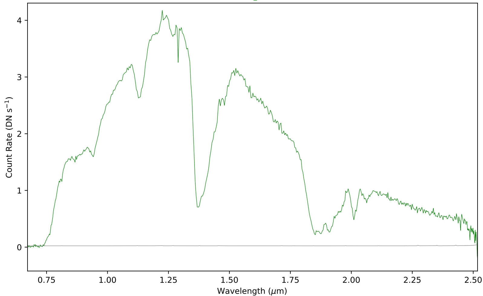
combspec2031-2048.fits - Aperture 1
