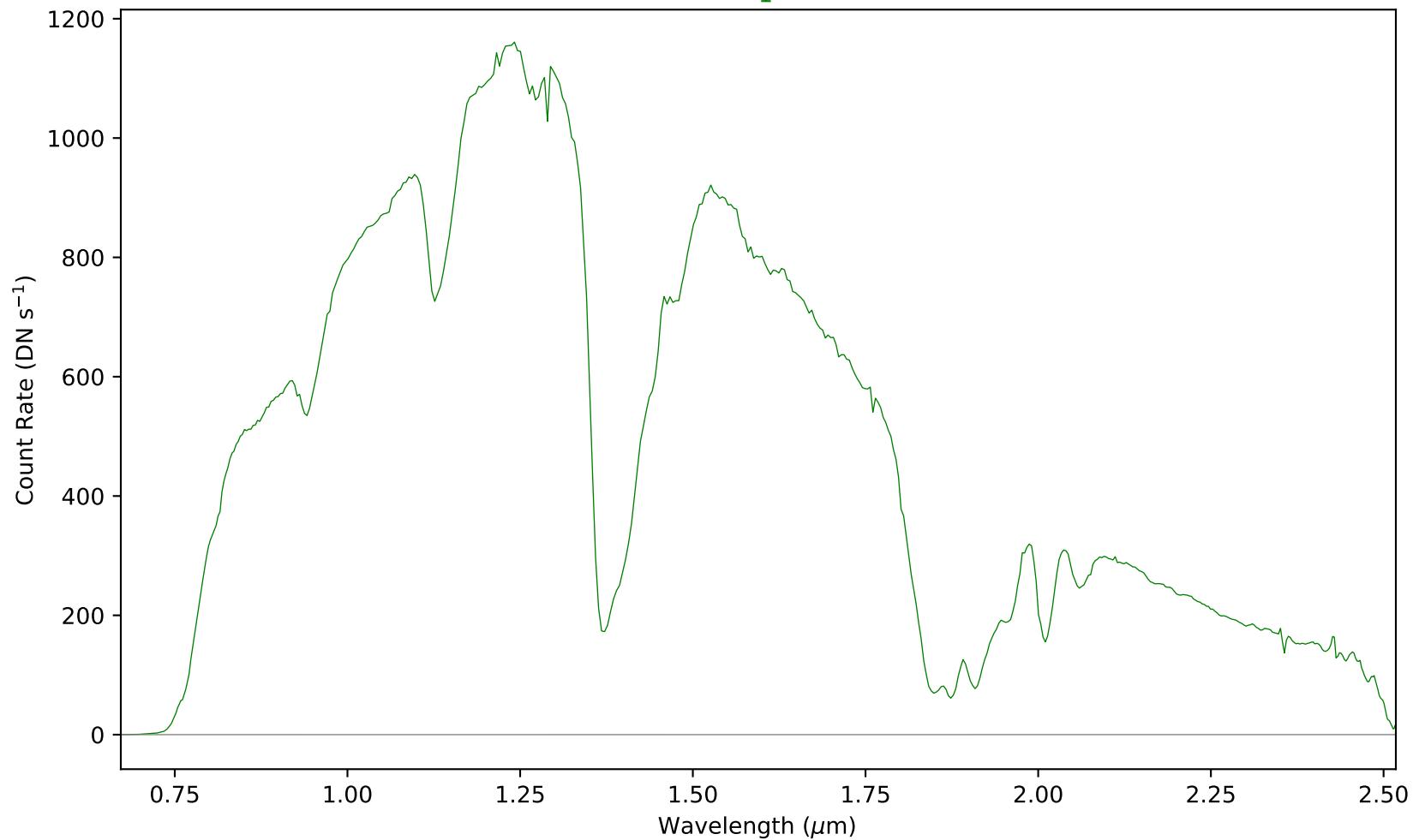
combspec2049-2062.fits - Aperture 1
