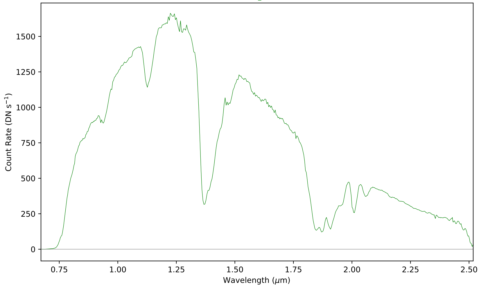
combspec2063-2072.fits - Aperture 1
