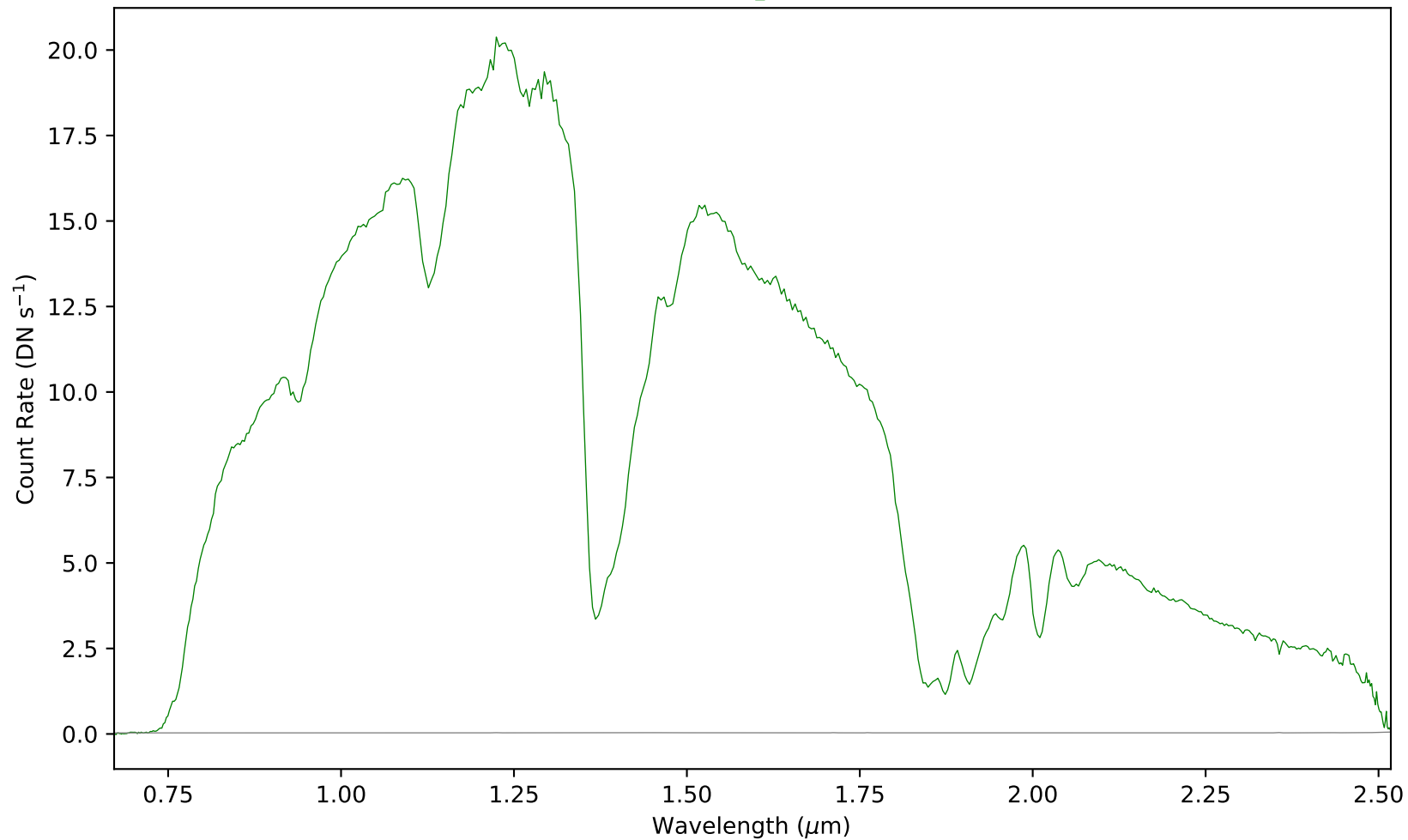
combspec2095-2108.fits - Aperture 1
