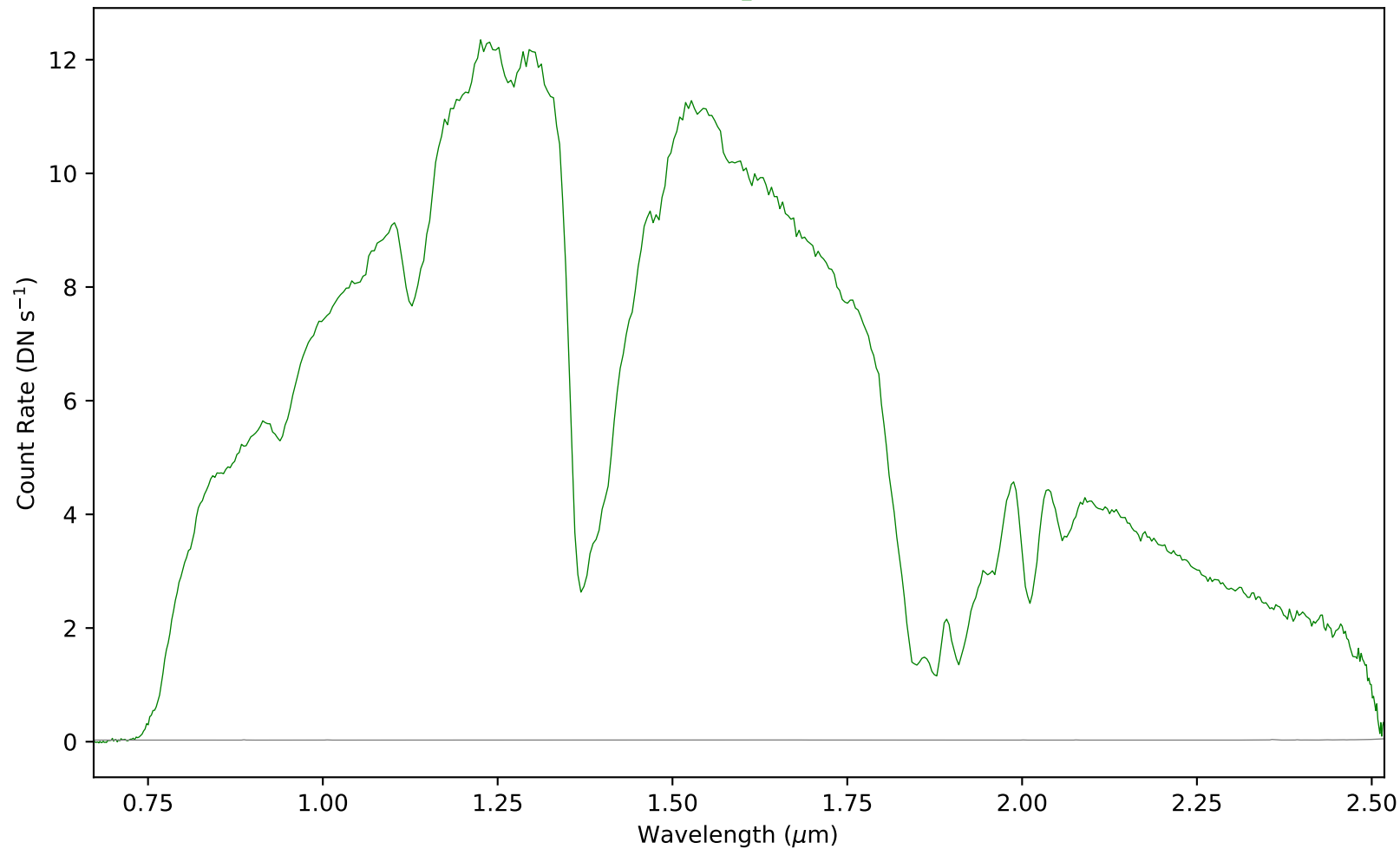
combspec2119-2134.fits - Aperture 1
