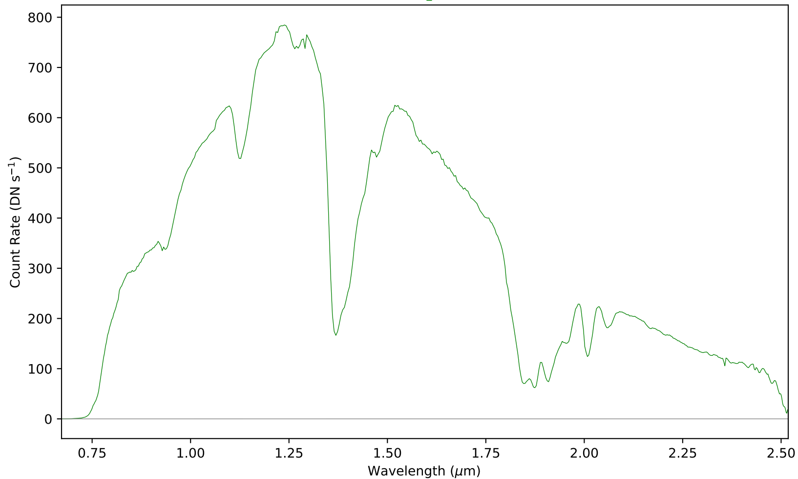
combspec2135-2144.fits - Aperture 1
