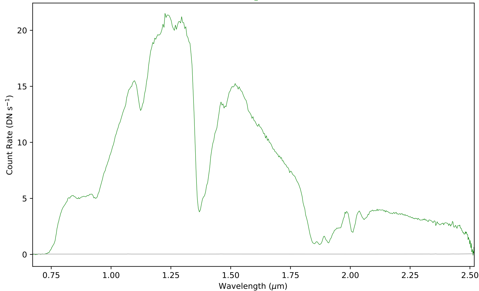
combspec2161-2174.fits - Aperture 1
