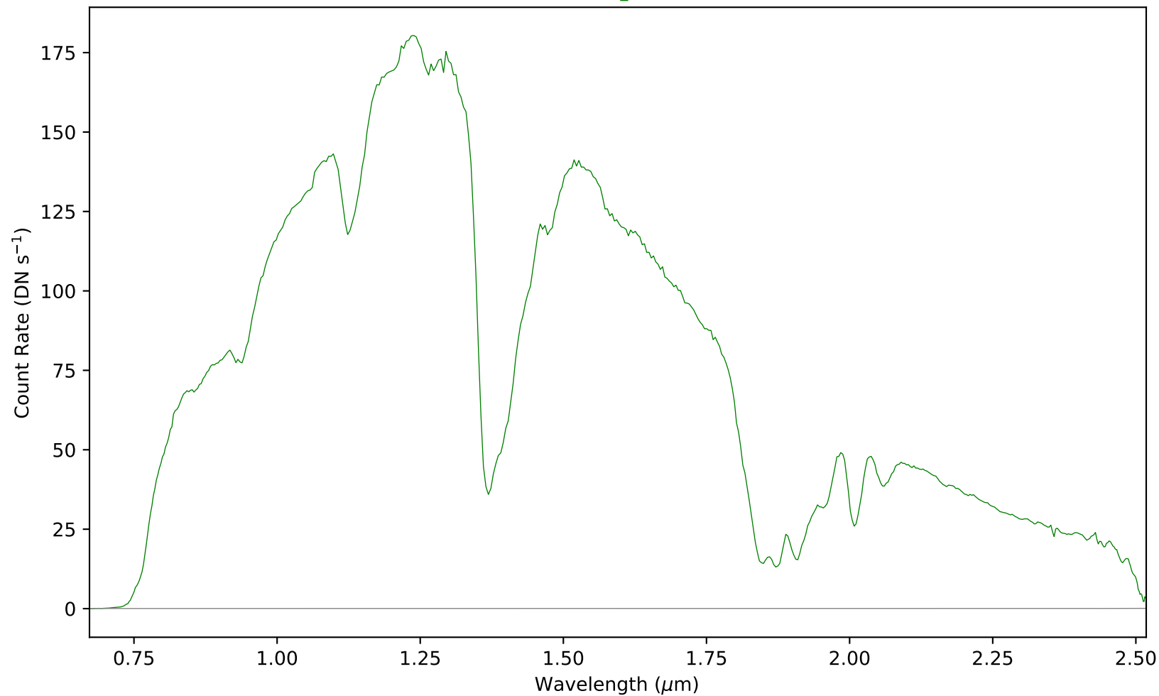
combspec2175-2184.fits - Aperture 1
