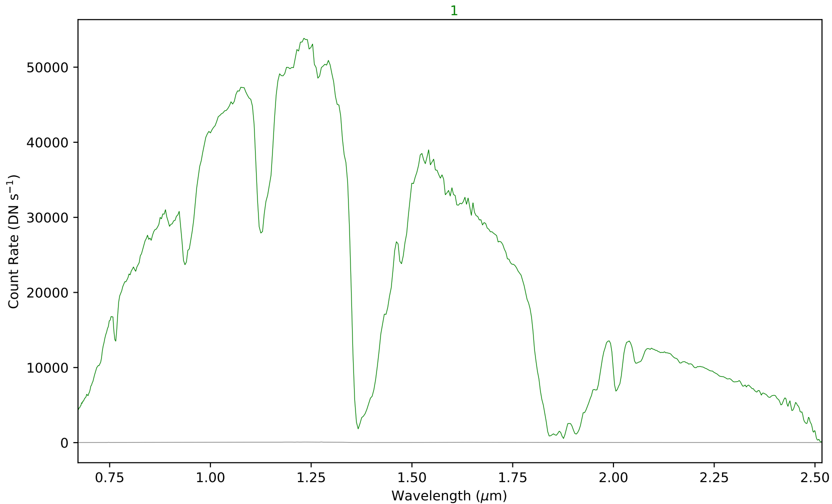
combspec1-6.fits - Aperture 1
