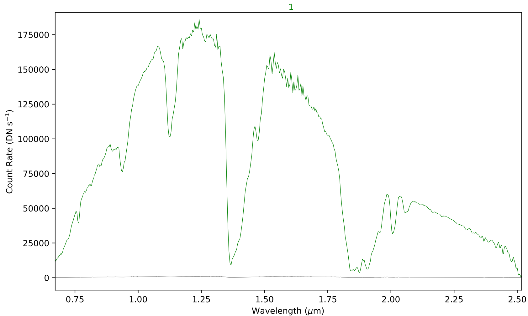
combspec111-114.fits - Aperture 1
