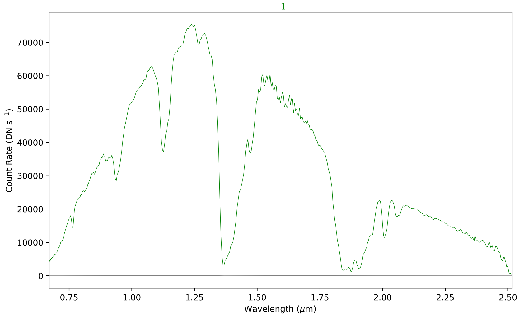
combspec13-50.fits - Aperture 1
