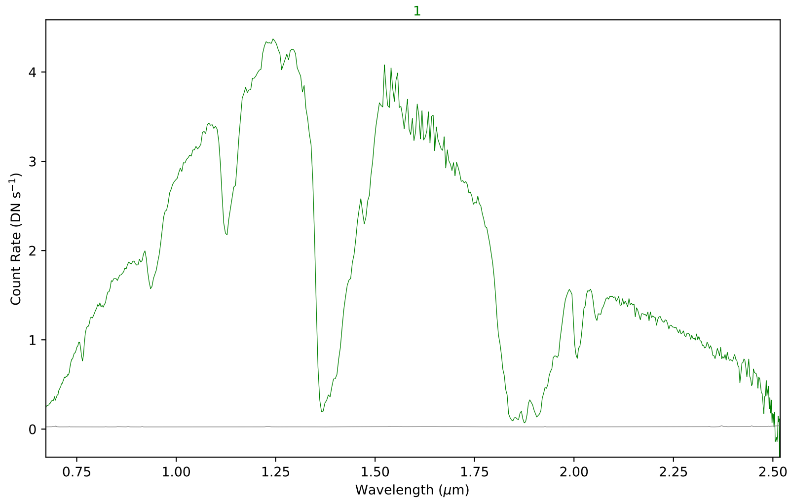
combspec165-184.fits - Aperture 1
