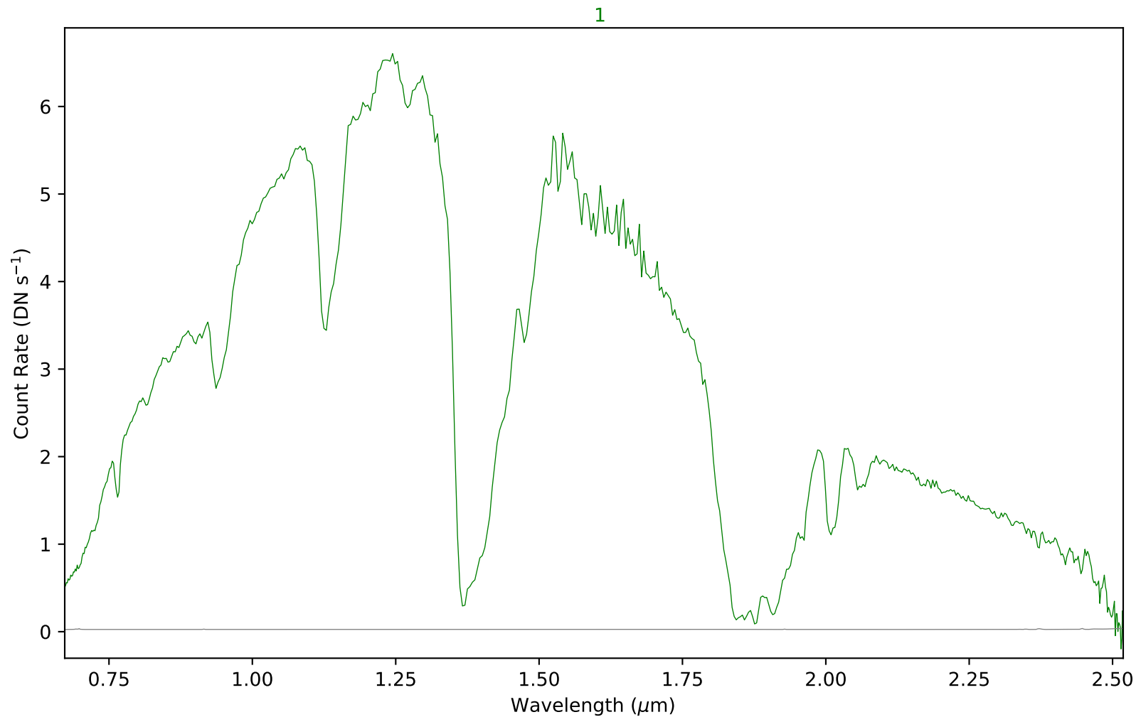
combspec197-216.fits - Aperture 1
