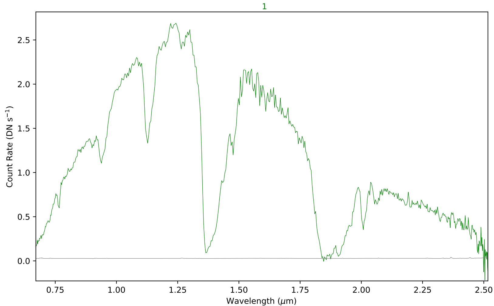
combspec25-44.fits - Aperture 1
