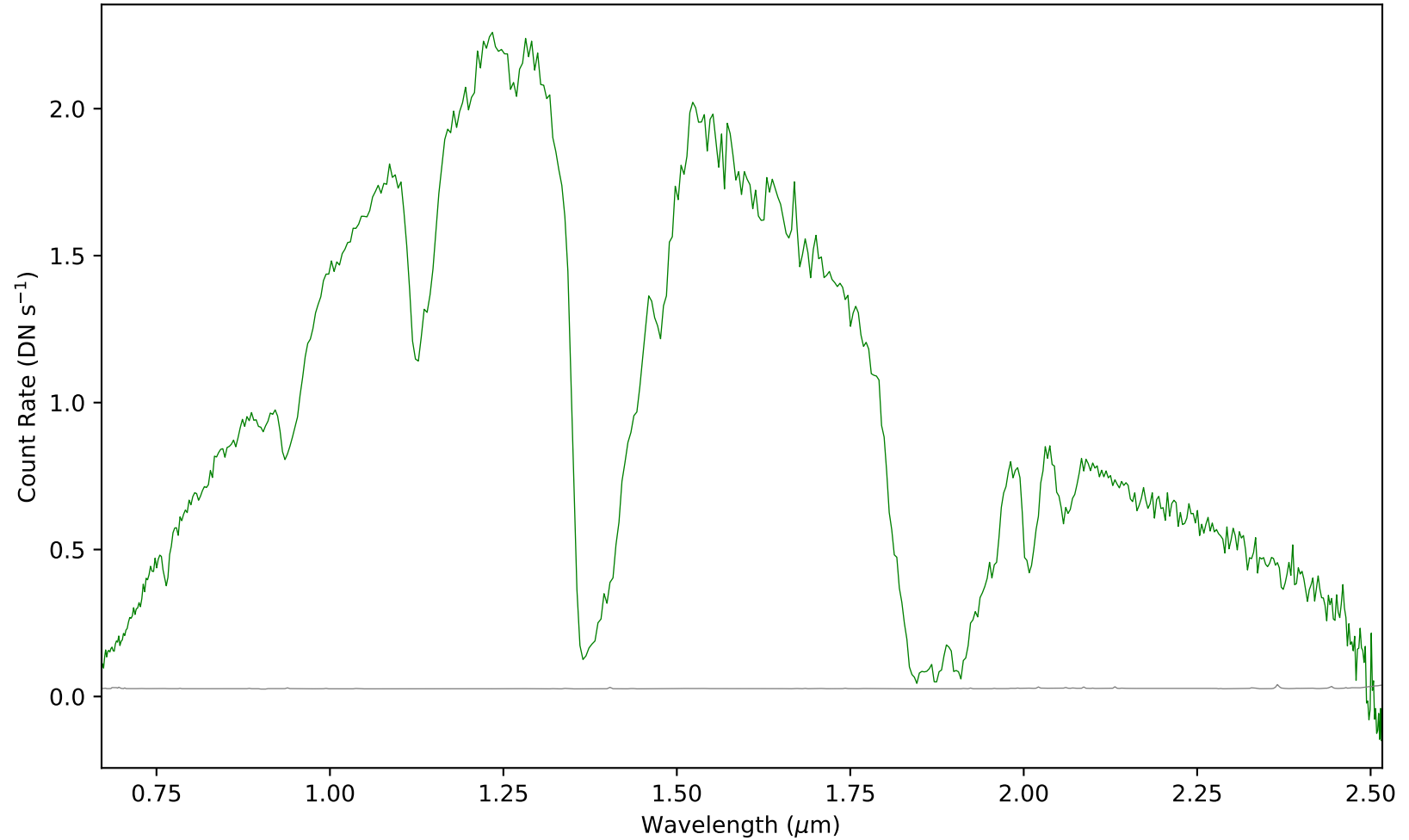
combspec57-76.fits - Aperture 1
