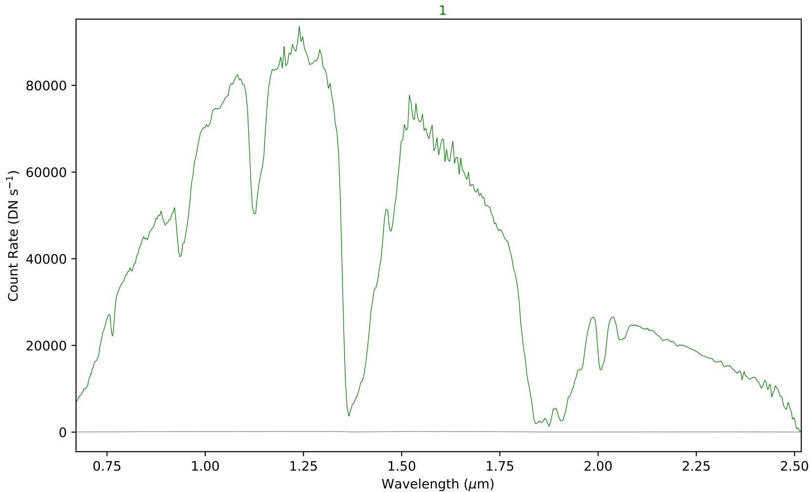
combspec77-82.fits - Aperture 1
