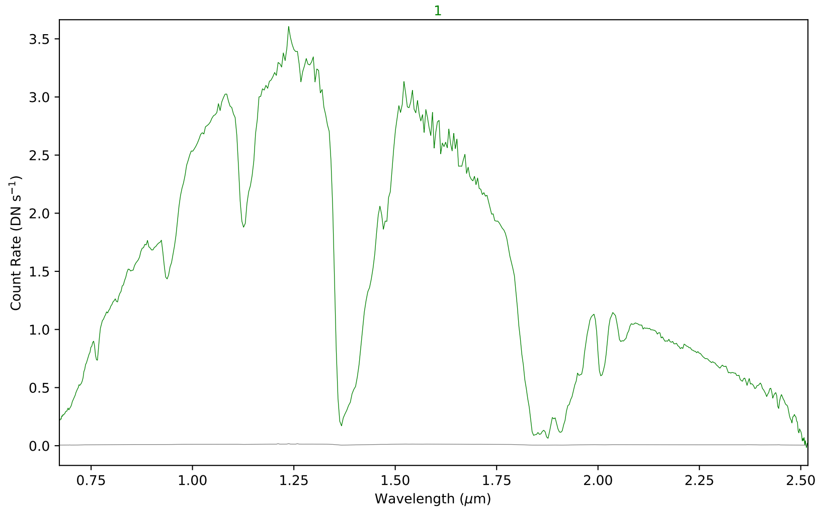
combspec89-110.fits - Aperture 1
