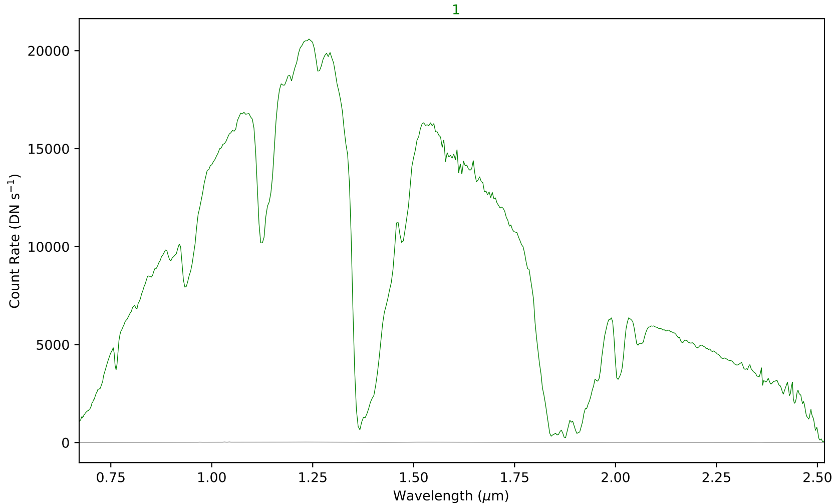
combspec283-288.fits - Aperture 1
