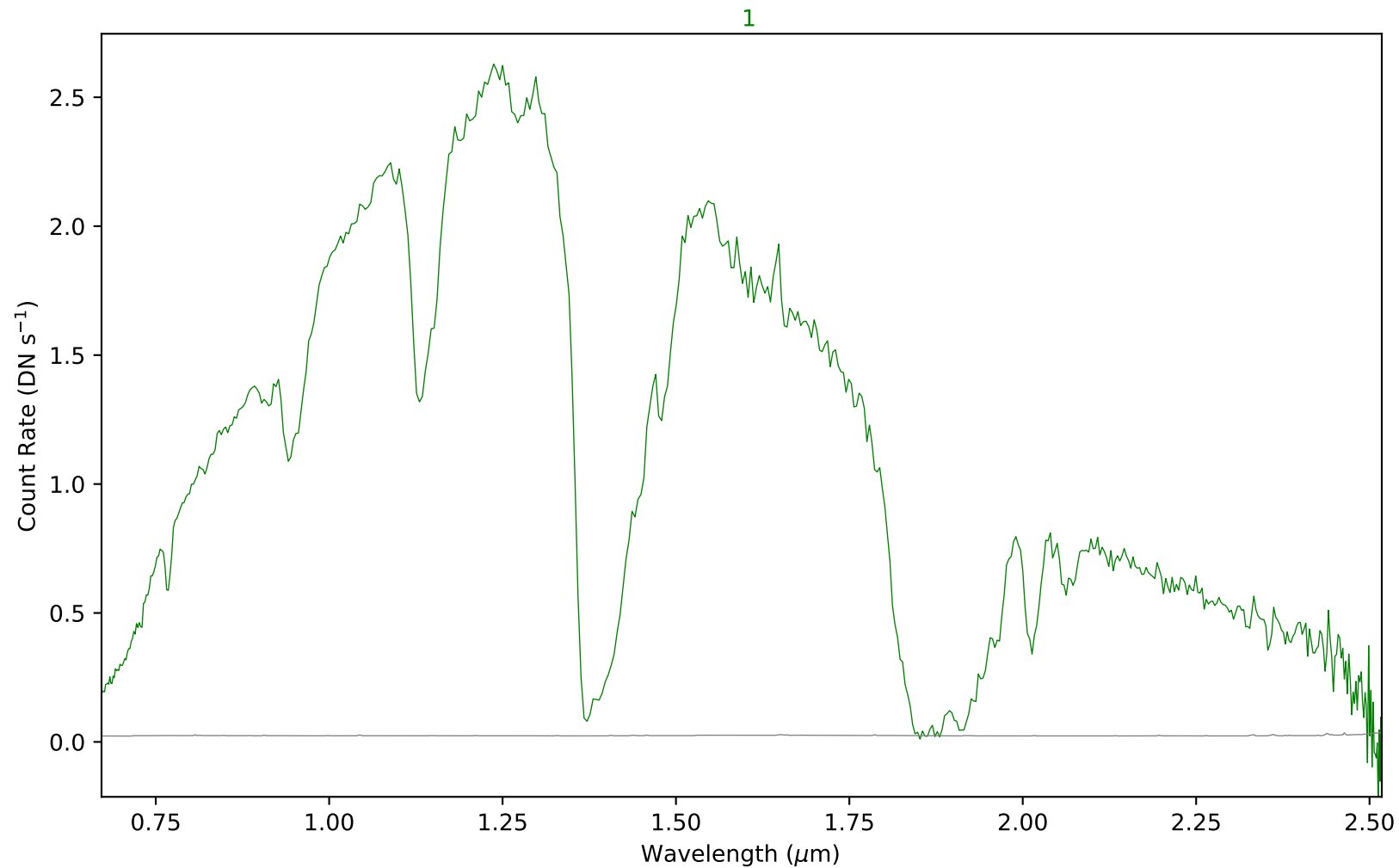
combspec307-326.fits - Aperture 1
