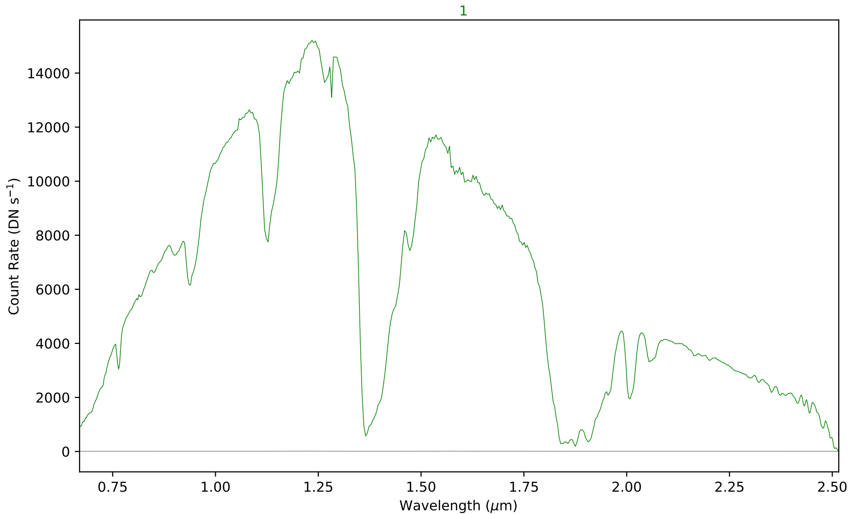
combspec383-388.fits - Aperture 1
