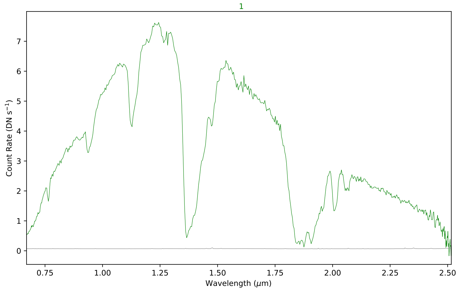
combspec446-455.fits - Aperture 1
