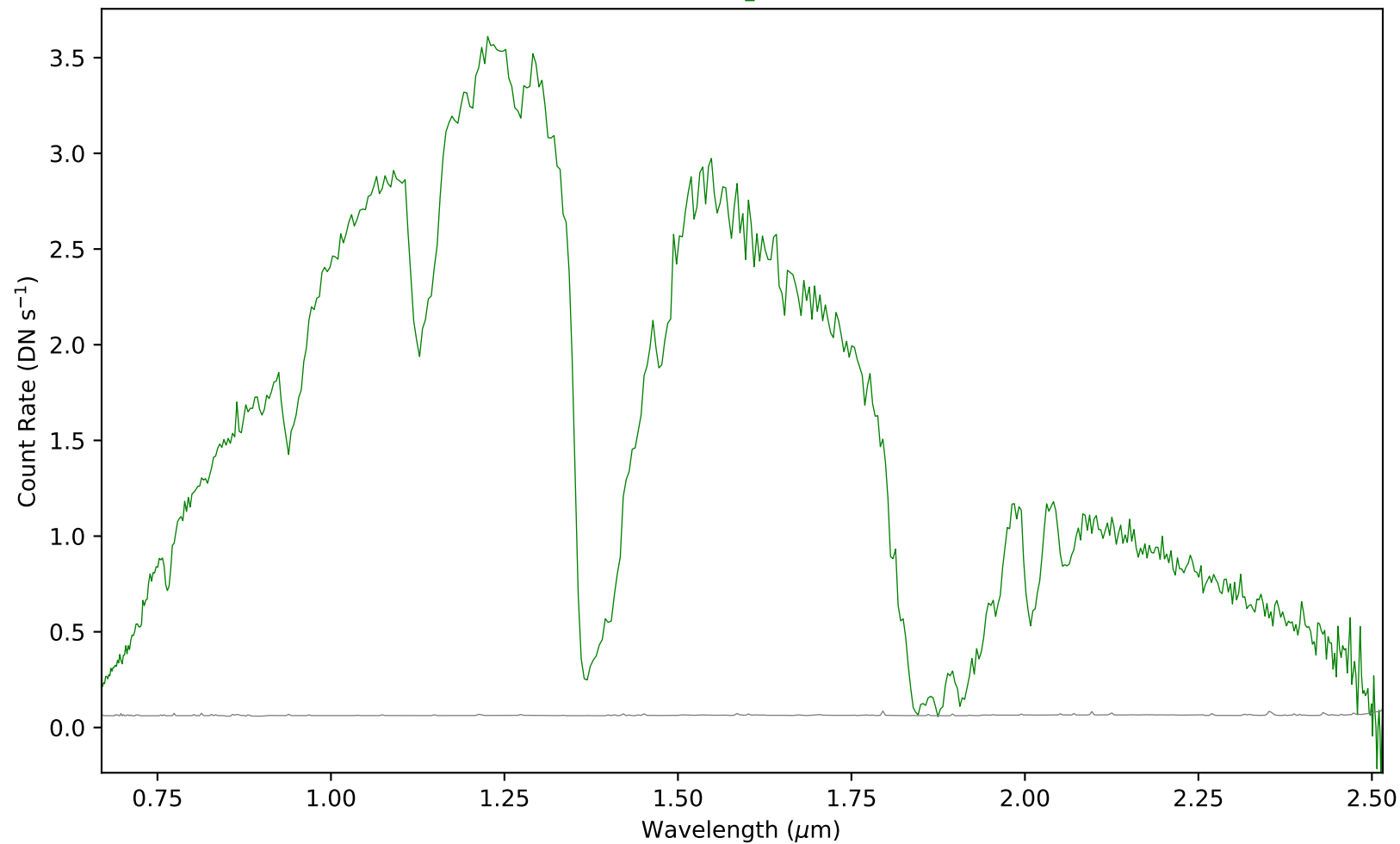
combspec474-483.fits - Aperture 1
