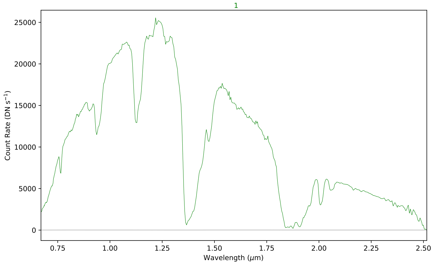
combspec462-467.fits - Aperture 1
