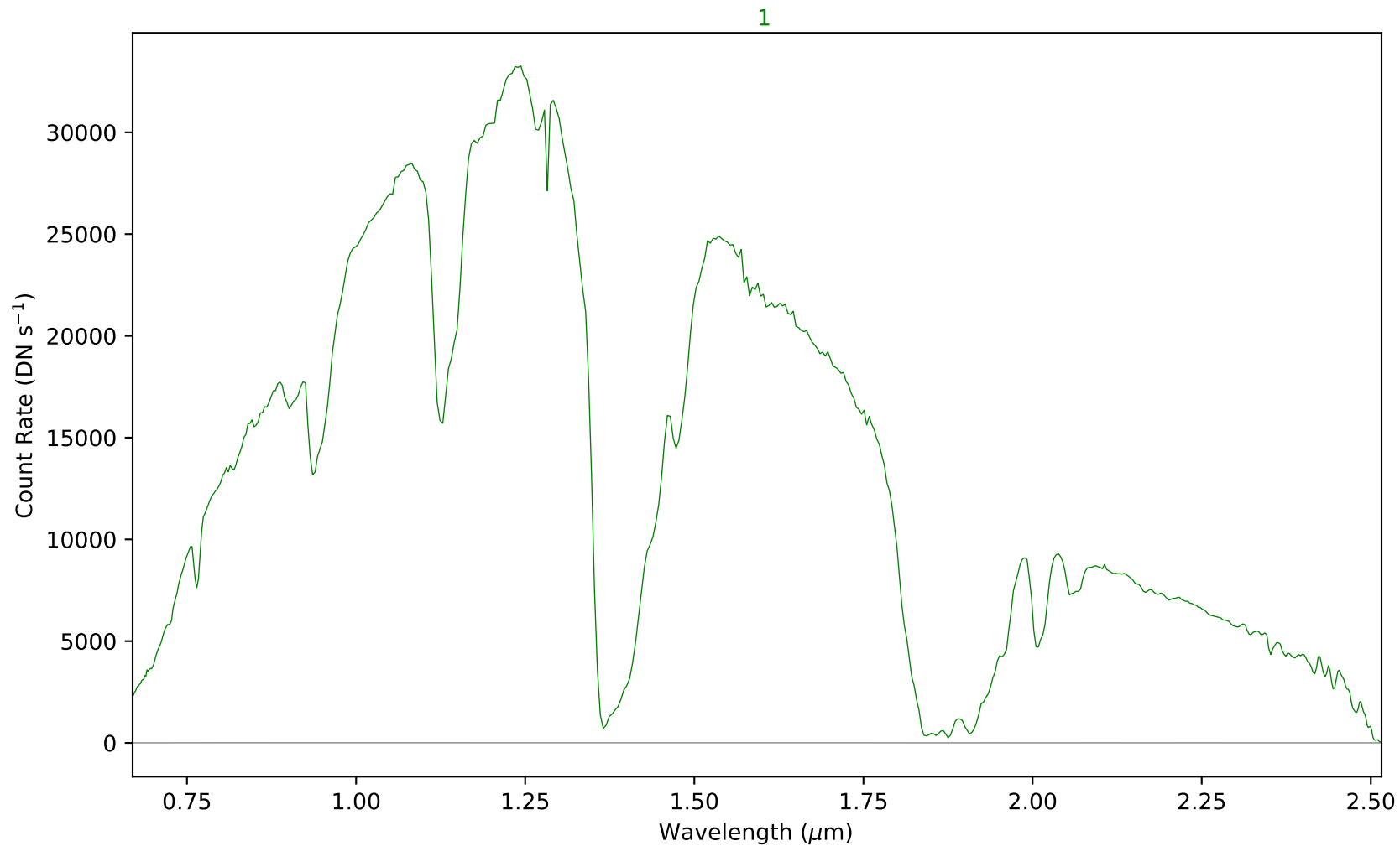
combspec575-592.fits - Aperture 1
