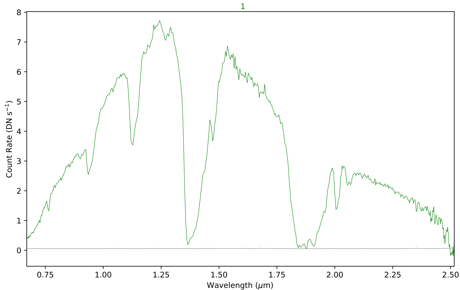
combspec599-608.fits - Aperture 1
