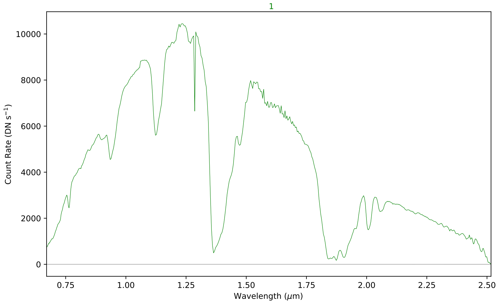
combspec647-734.fits - Aperture 1
