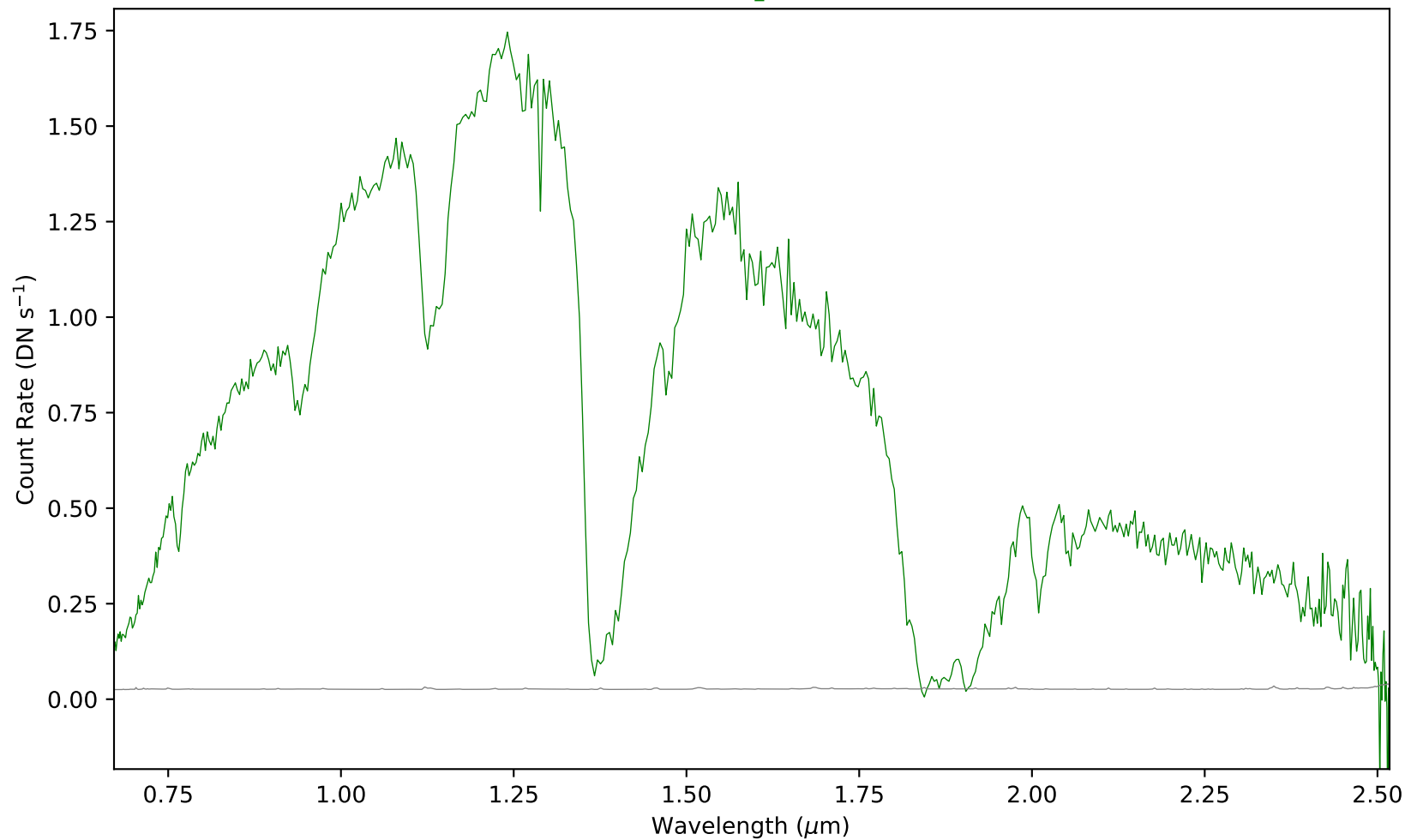
combspec695-728.fits - Aperture 1
