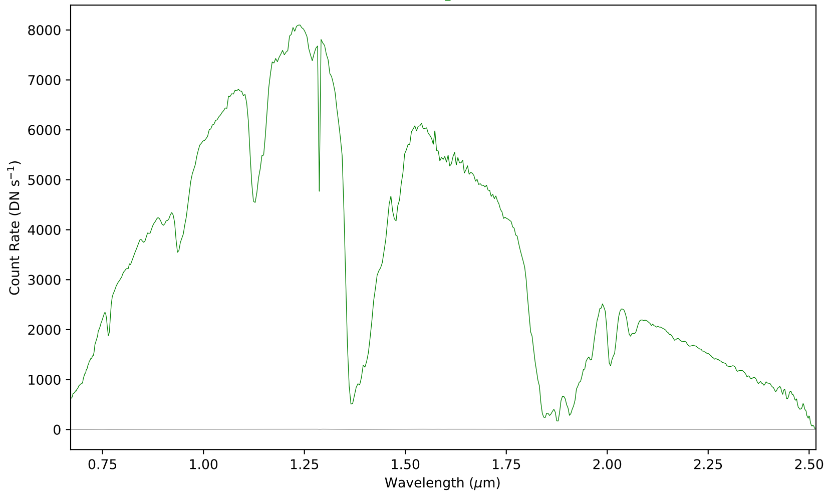
combspec741-746.fits - Aperture 1
