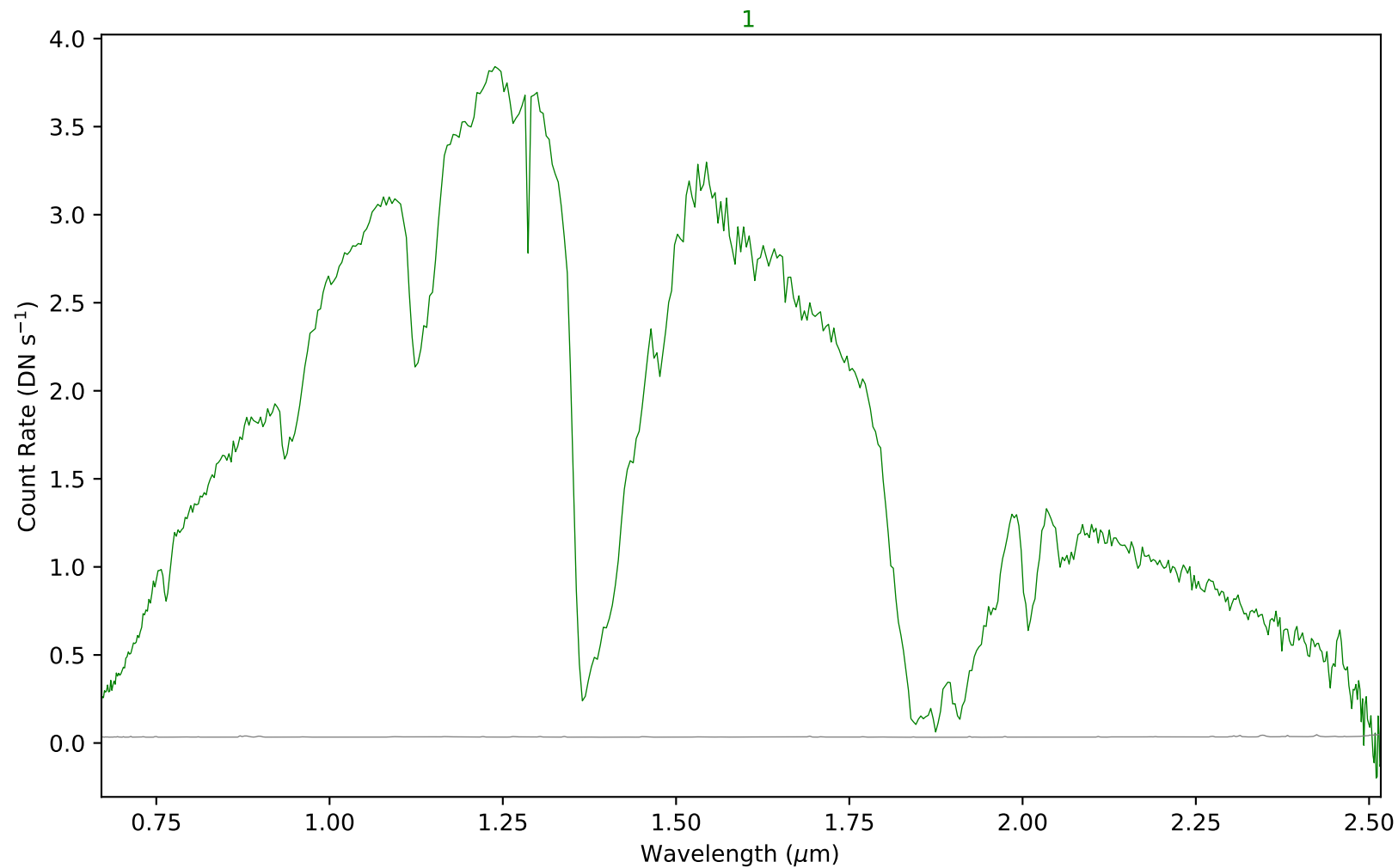
combspec753-834.fits - Aperture 1
