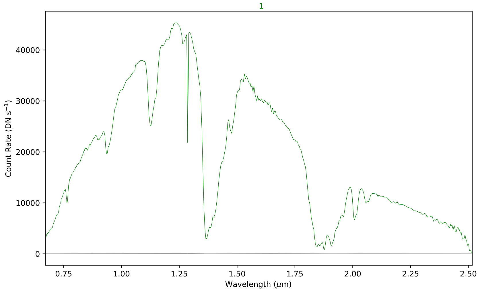
combspec765-770.fits - Aperture 1
